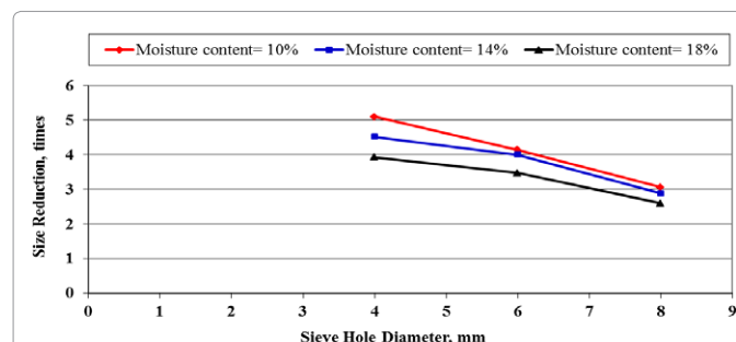
Figure 8: Effect of moisture content and sieve holes diameter on sizedreduction.
